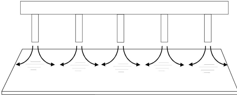
Illustration #2 Tempering Quench Jets Showing Non-Uniform Flow
